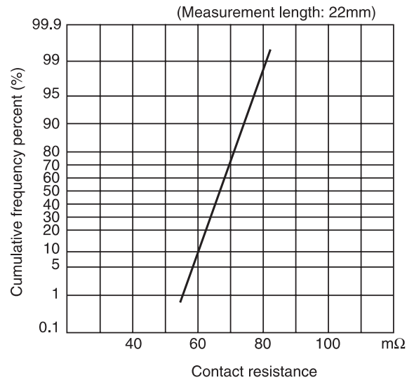
(2) Contact resistance
