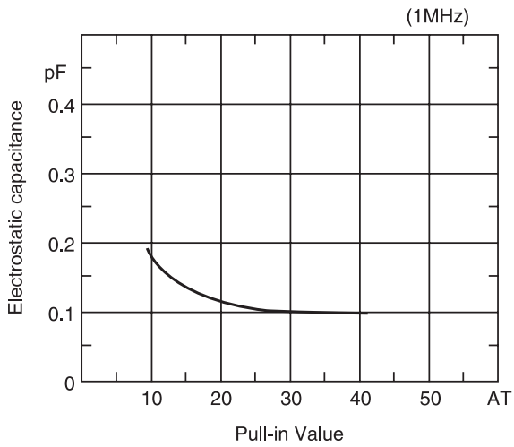
(5) Electrostatic capacitance
