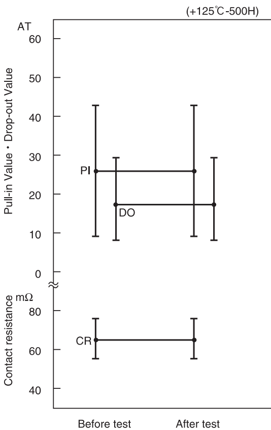
(4) High temperature storage test
