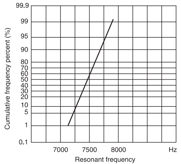
(4) Resonant frequency
