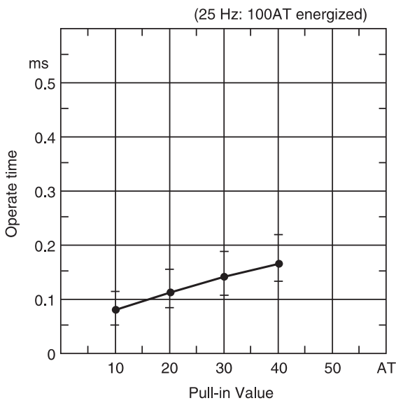
(1) Operate time
