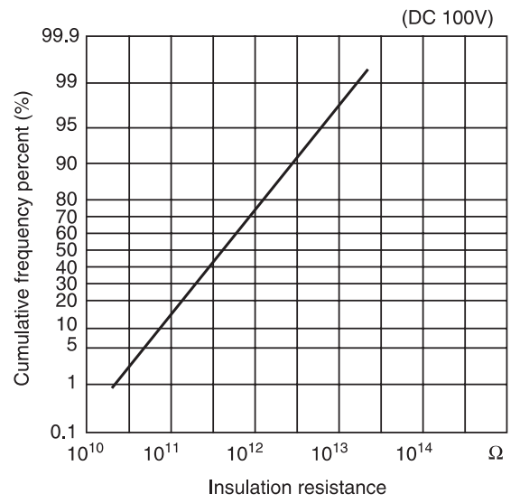
(4) Insulation resistance
