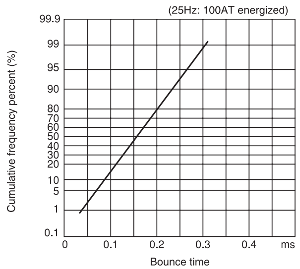
(2) Bounce time
