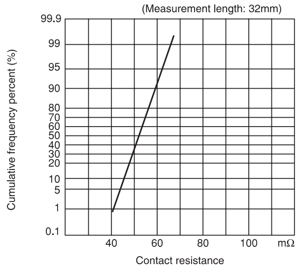
(2) Contact resistance
