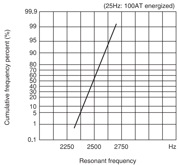
(4) Resonant frequency
