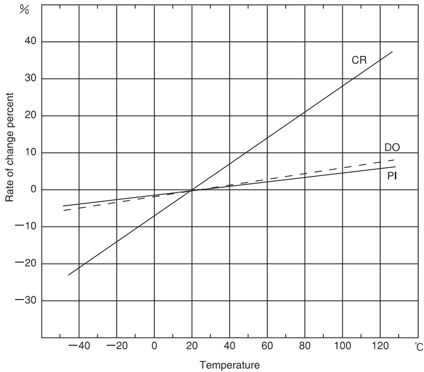
(1) Temperature characteristics
