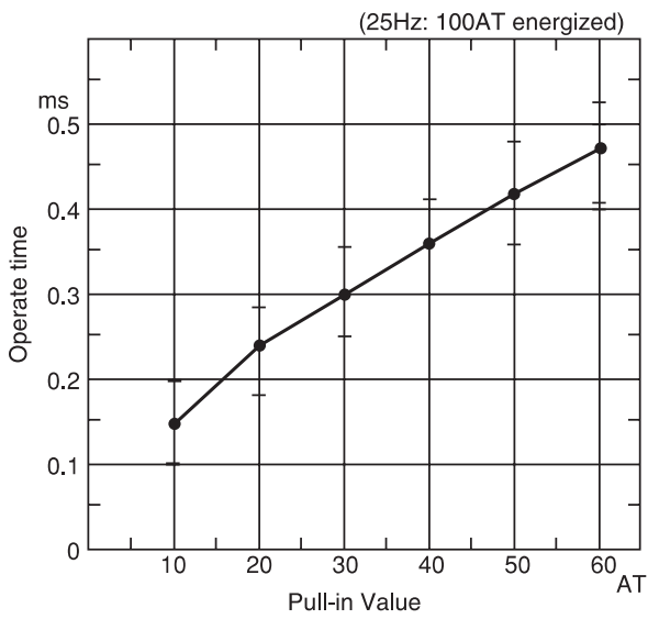
(1) Operate time
