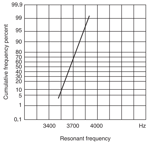
(4) Resonant frequency
