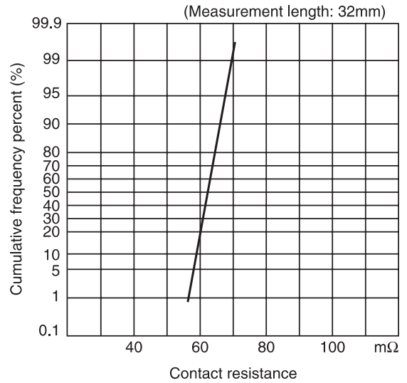
(2) Contact resistance
