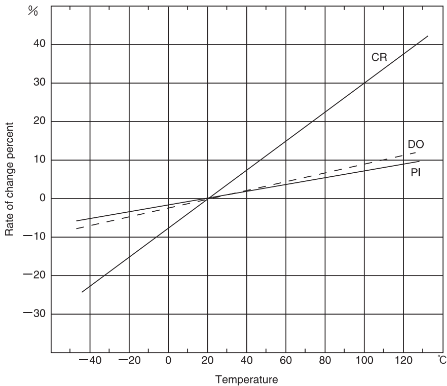
(1) Temperature characteristics
